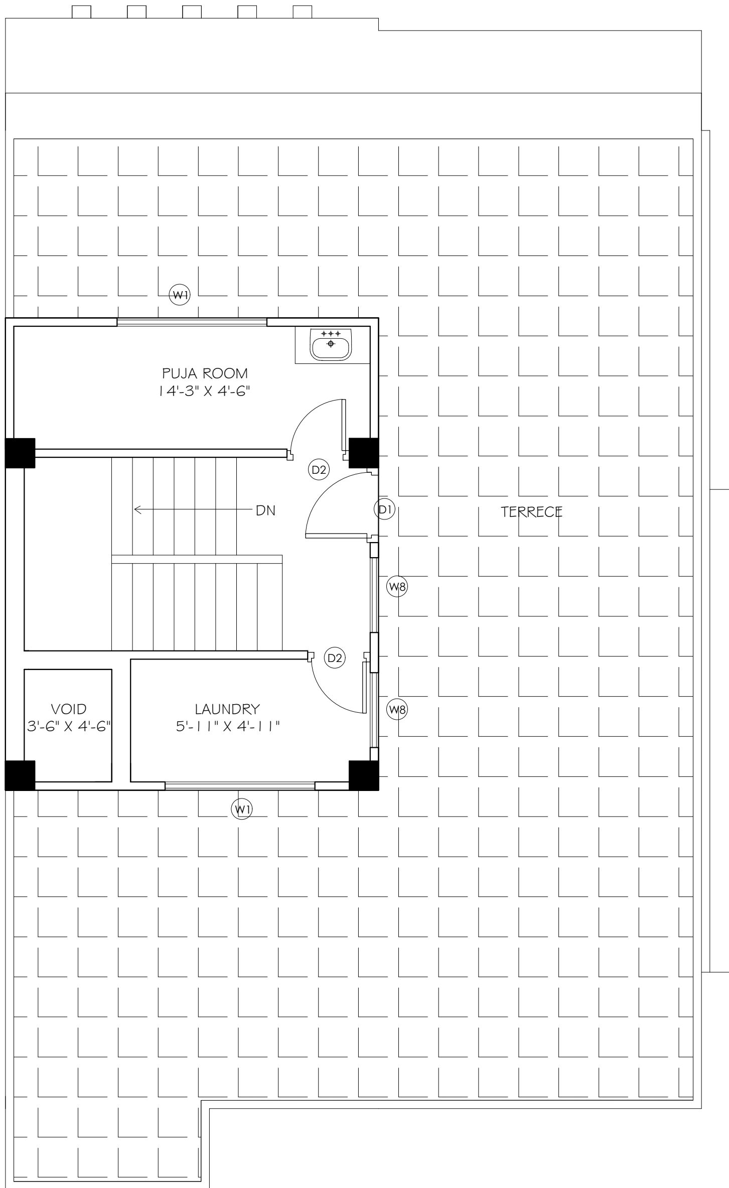
TOP FLOOR PLAN FOR COUNTABLE AREA:-282.51 SQ.FT. FOR NON COUNTABLE AREA:-0 SQ.FT TOTAL AREA:-282.51 SQ.FT.
